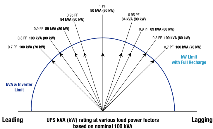
Chloride UPS 3-phase systems will support any load power factor without de-rating
